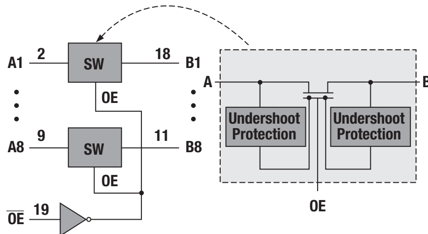
CBT3245 Logic Diagram
