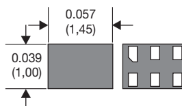
6-Pin Micro QFN (DRY)
