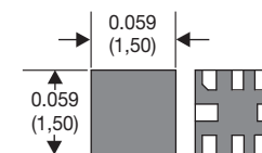
8-Pin QFN (RSE)
